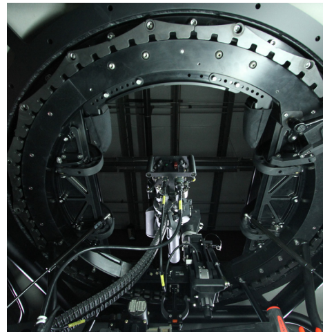
Deployed M134D in a CEV System - view from inside
