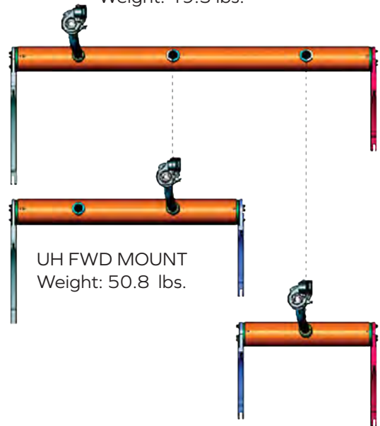
UH AFT MOUNT Weight: 42.8 lbs.
